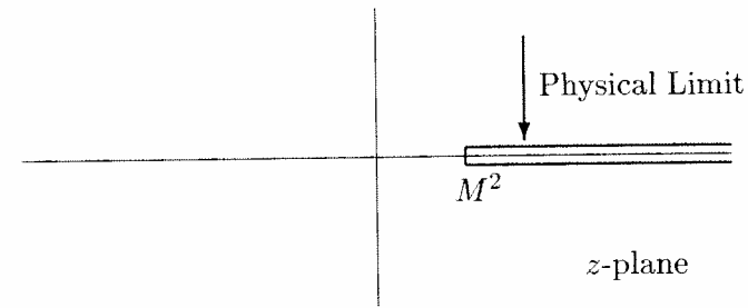
Fig. 6.2. Analytic structure of the Green's function.
