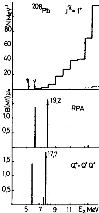
Fig.1. The M1 resonance in ^{208}\text{Pb} . The histogram of the number of two-phonon states in the energy interval of 1 MeV (the positions of the 1p - 1h states (1i_{11/2}^{-1} 1i_{13/2}^{-1}) and (1h_{9/2}^{-1} 1h_{11/2}^{-1}) are indicated by arrows) is shown in the upper part of the figure. The results of calculations in the RPA and with the inclusion of interaction between one- and two-phonon states are shown in the middle and lower parts of the figure respectively.
