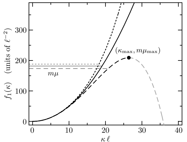
FIG. 7: Right hand side f_1(\kappa) of the extremum condition (63) as function of the Fermi momentum for a noninteracting single-component gas (solid), with repulsive p-wave interaction a_1/\ell = 0.04 (dotted), and with attractive p-wave interaction a_1/\ell = -0.04 (dashed). The horizontal lines mark the respective values of the chemical potentials for N = 10^6 particles.
