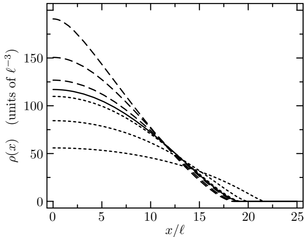
FIG. 5: Density profile \rho(x) of a single-component Fermi gas of N = 10^6 particles trapped in a spherical symmetric parabolic trap with oscillator length \ell . The solid curve shows the noninteracting gas a_1/\ell = 0 . Dotted curves correspond to repulsive p-wave interactions with a_1/\ell = 0.03, 0.06 , and 0.1 (from top to bottom). The dashed curves show attractive p-wave interactions with a_1/\ell = -0.03, -0.04 and -0.044 (top to bottom), respectively.
