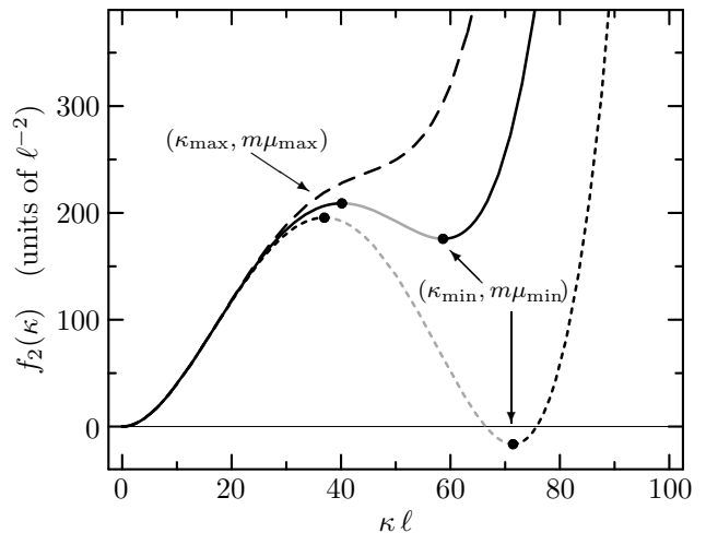
FIG. 9: Right hand side f_2(\kappa) of the extremum condition (74) as function of the Fermi momentum for attractive s-wave interaction with a_0/\ell = -0.05 and a repulsive p-wave interaction with \tilde{a}_1/\ell = 0.014 (dotted curve), 0.015 (solid), and 0.016 (dashed). The gray segments of the curves correspond to maxima of the energy density.
