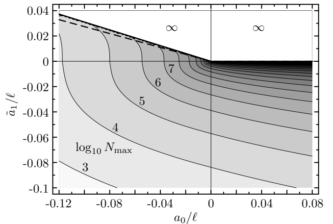
FIG. 8: Contour plot of the logarithm of the maximum particle number, \log_{10} N_{\max} , as function of the s- and p-wave scattering lengths for a two-component Fermi gas in a harmonic oscillator potential with mean oscillator length \ell . Selected contours are labeled with the corresponding value of \log_{10} N_{\max} . In the white area at positive p-wave scattering length no collapse can occur, i.e., the maximum particle number is infinity.
