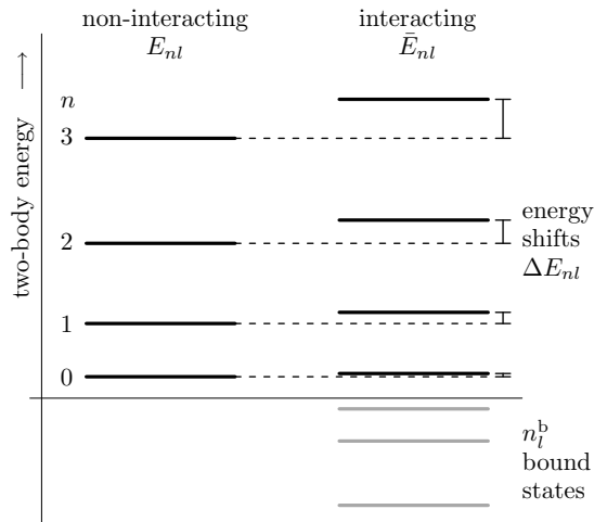
FIG. 1: Schematic comparison of the free two-body energy spectrum E_{nl} with the energy spectrum \bar{E}_{nl} in presence of a two-body interaction for given relative angular momentum l . The interaction generates n_l^b bound states and shifts the positive energy states by \Delta E_{nl} .
