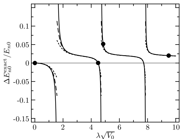
FIG. 3: Relative energy-shift \Delta E_{n0}^{\text{exact}}/E_{n0} obtained from the exact l = 0 solutions plotted versus the strength \lambda\sqrt{V_0} of the square-well potential. The solid line gives the energy shift for the lowest ( n = 1 ), the dashed line for the 10th, and the dotted line for 20th state of the positive energy spectrum. The dots mark the interaction strengths used in Fig. 2.
