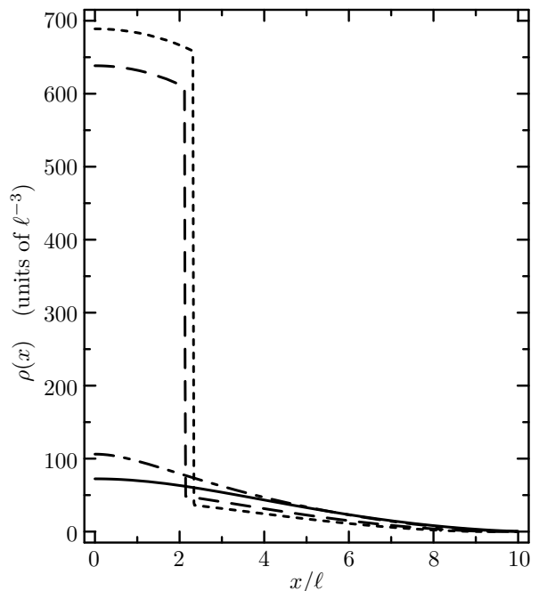
FIG. 11: Evolution of the density profile of a two-component system of N = N_1 = N_2 = 60000 particles with p-wave scattering length \tilde{a}_1/\ell = 0.03 according to the Gedankenexperiment described in the text. The s-wave scattering length is tuned in the range a_0/\ell = -0.095 (solid), -0.1 (dash-dotted), -0.101 (dashed), and -0.102 (dotted).
