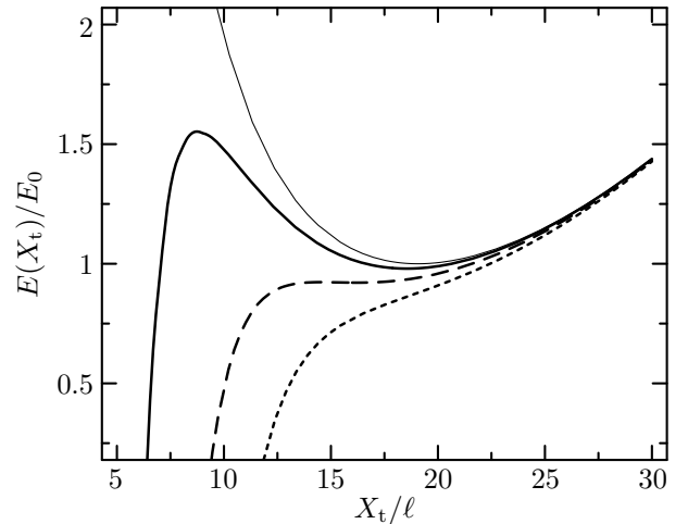
FIG. 6: Variational energy (65) of a trapped single-component Fermi gas with N = 10^6 as function of the parameter X_t . The curves show the noninteracting gas (thin solid), a_1/\ell = -0.035 (solid), a_1/\ell = -0.051 (dashed), and a_1/\ell = -0.065 (dotted). The energies are given in units of the ground state energy E_0 of the noninteracting gas.
