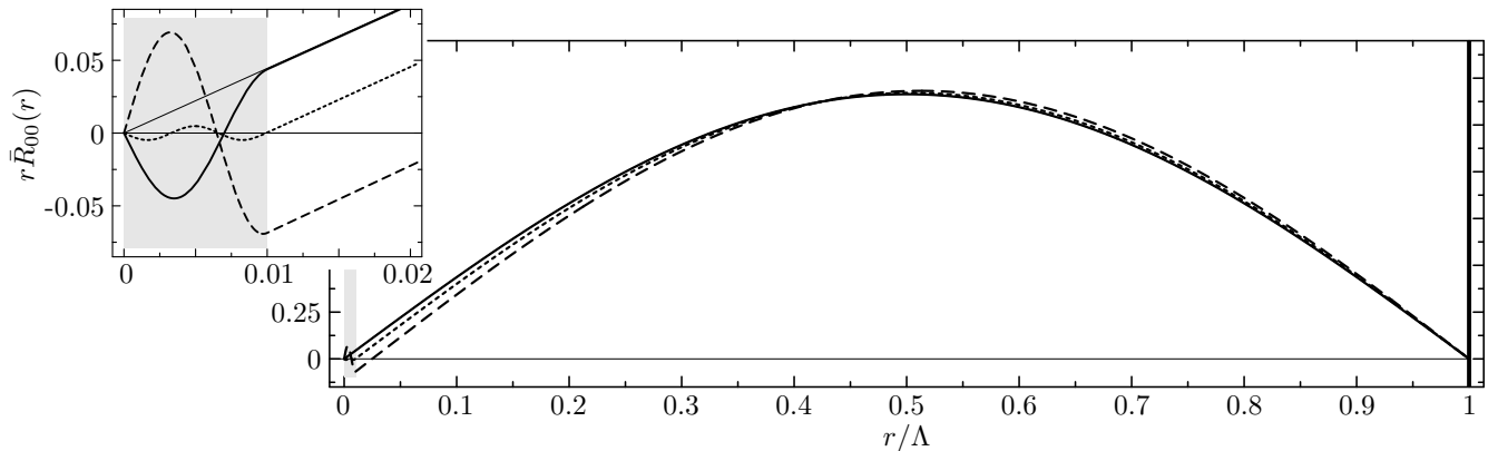
FIG. 2: Radial wave functions r\bar{R}_{00}(r) of the lowest l = 0 positive energy state for different potential depths V_0 of the square-well potential. The interaction strengths are \lambda\sqrt{V_0} = 0 (thin solid), 4.49 (solid), 4.85 (dashed), and 9.5 (dotted). The radius of the well is \lambda = 0.01\Lambda and marked by the gray area. The insert shows a magnification of the region around the origin.
