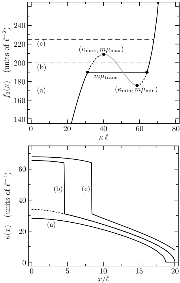
FIG. 10: Upper plot: f_2(\kappa) of the extremum condition (74) as function of the Fermi momentum for an interaction with a_0/\ell = -0.05 and \tilde{a}_1/\ell = 0.015 . Lower plot: Distribution of local Fermi momenta \kappa(x) for a spherical trap of oscillator length \ell for the three different chemical potentials marked in the upper panel. Solid curves show the equilibrium profiles, dotted curves show metastable configurations.
