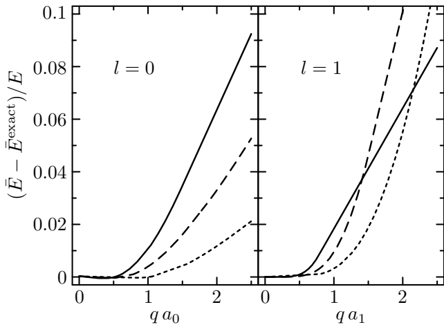
FIG. 4: Relative deviation of the two-body energy calculated with the ECI in scattering length approximation from the exact energy as function of qa_l for l = 0 (left) and l = 1 states (right). The curves were obtained for interactions with three bound states by varying the strength \lambda\sqrt{V_0} and looking at the energy shifts for different relative momenta q_{nl}\Lambda \approx 20 (solid), 40 (dashed), and 80 (dotted).
