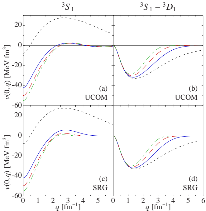
FIG. 2: (color online) Off-diagonal matrix elements v(0, q) in the {}^3S_1 and {}^3S_1 - {}^3D_1 partial waves. Panels (a) and (b) show the V_{\text{UCOM}} matrix elements for I_\vartheta = 0.03 \text{ fm}^3 (—), 0.06 \text{ fm}^3 (---), and 0.09 \text{ fm}^3 (- - -) in comparison to those of AV18 (----). Panels (c) and (d) show the SRG-evolved matrix elements of V_\alpha for flow parameter values \bar{\alpha} = 0.0055 \text{ fm}^4 (—), 0.0125 \text{ fm}^4 (---), and 0.0215 \text{ fm}^4 (- - -), which have been chosen to reproduce the value of the corresponding V_{\text{UCOM}} matrix element at q = q' = 0 \text{ fm}^{-1} .
