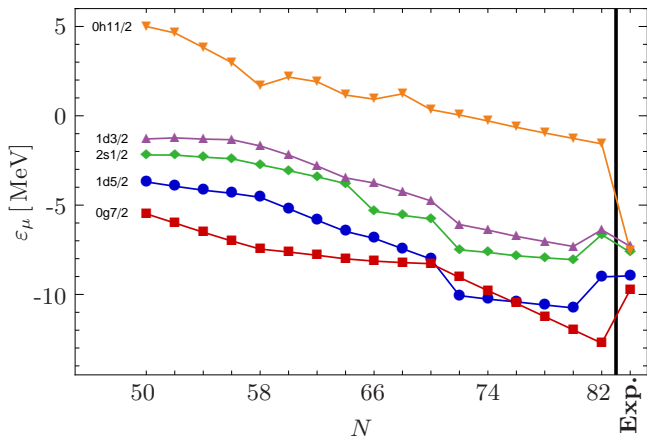
FIG. 10: (Color online) Corrected canonical neutron single-particle energies in the tin isotopes, calculated for a V_{UCOM} with \bar{\alpha} = 0.04 \text{ fm}^4 . Experimental single-particle energies of ^{132}\text{Sn} (“Exp.”) are included for reference [57].
