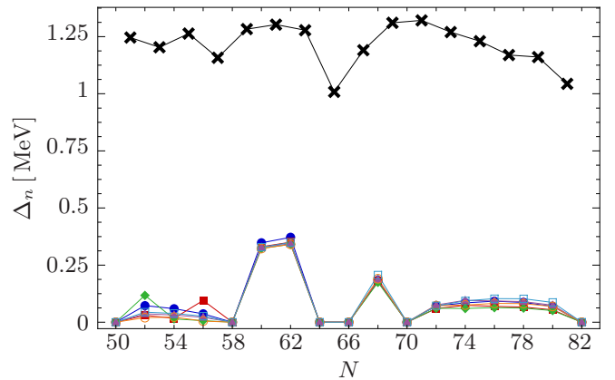
FIG. 9: (Color online) Canonical gaps in the tin isotopes for V_{\text{UCOM}} with \bar{\alpha} = 0.03 (●), 0.04 (■), 0.05 (◆), 0.06 (▲), 0.08 (○), and 0.1 \text{ fm}^4 (□), compared to experimental \Delta^{(3)}(N) (×) [46].
