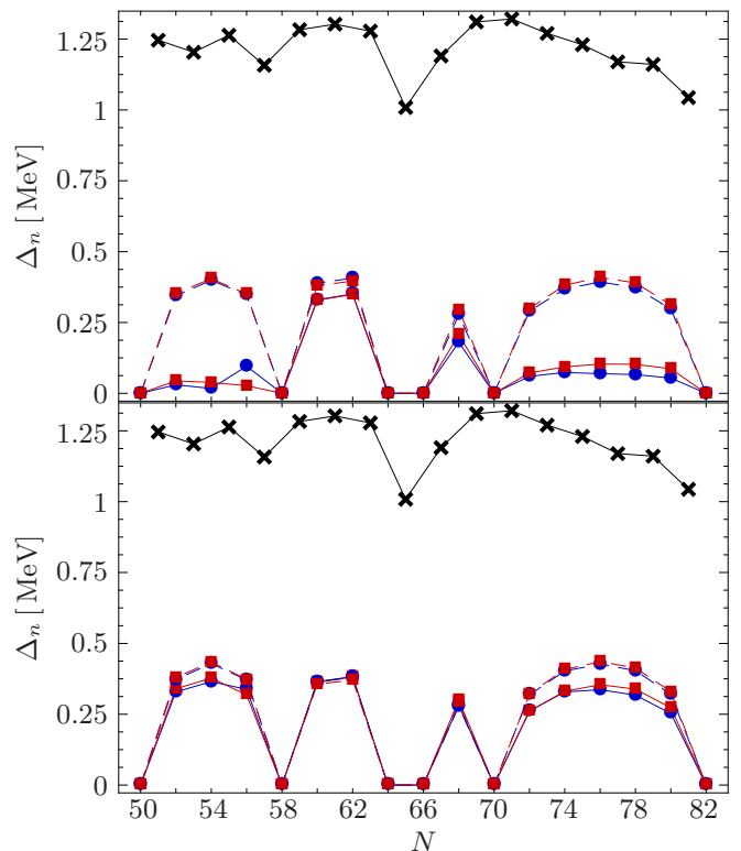
FIG. 11: (Color online) Canonical (top) and average gaps (bottom) of tin isotopes for V_{UCOM} with \bar{\alpha} = 0.04 (●), and 0.1 \text{ fm}^4 (■). Comparison of full interaction (solid) and ^1S_0 partial wave (dashed). Experimental \Delta^{(3)}(N) are indicated by (X) [46].
