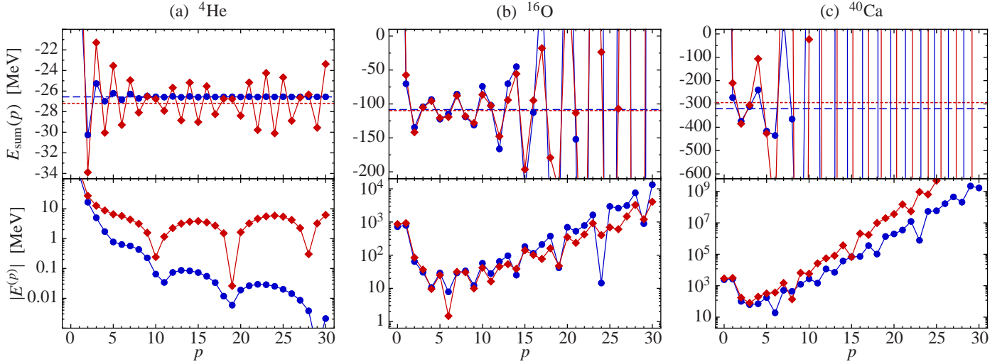
Figure 1: Contributions to the ground-state energies in MBPT up to 30th order for different nuclei and model spaces: (a) {}^4\text{He} in a 12\hbar\Omega model space with \hbar\Omega = 20 MeV (●) and 32 MeV (◆); (b) {}^{16}\text{O} in 6\hbar\Omega with \hbar\Omega = 20 MeV (●) and 24 MeV (◆); (c) {}^{40}\text{Ca} in 4\hbar\Omega with \hbar\Omega = 20 MeV (●) and 24 MeV (◆). The upper panels depict the partial sum E_{\text{sum}}(p) defined in Eq. (12) as function of the largest order p , the lower panels the modulus of the individual contributions E^{(p)} on a logarithmic scale. The dashed horizontal lines in the upper panels indicate the NCSM ground-state energies for the respective nuclei and model spaces.
