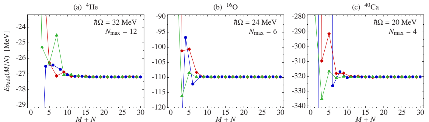
Figure 2: Padé approximants for the ground-state energies of (a) {}^4\text{He} , (b) {}^{16}\text{O} , and (c) {}^{40}\text{Ca} as function of the summed order M+N . The different symbols represent the diagonal approximants E_{\text{Padé}}(M/M) (●), the super-diagonal approximants E_{\text{Padé}}(M-1/M) (◆), and the sub-diagonal approximants E_{\text{Padé}}(M/M-1) (▲). The model space size N_{\text{max}} and the oscillator frequency \hbar\Omega is quoted in the individual panels. The dashed horizontal lines indicate the NCSM ground-state energies for the respective nuclei and model spaces.
