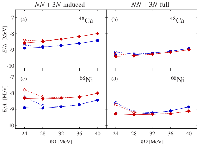
FIG. 1: (Color online) Comparison of CCSD ground-state energies at flow parameters \alpha = 0.04 \text{ fm}^4 (blue circles) and 0.08 \text{ fm}^4 (red diamonds), without (open symbols) and with (full symbols) frequency conversion, using E_{3\text{max}} = 14 and e_{\text{max}} = 12 . The frequency conversion was performed using the parent frequency \hbar\Omega_{\text{SRG}} = 36 \text{ MeV} .
