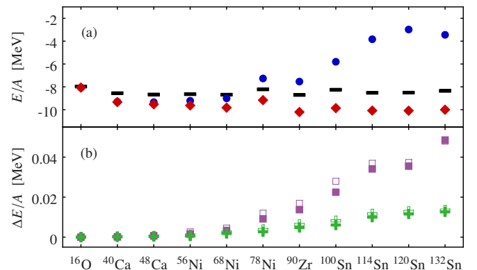
FIG. 2: (Color online) (a) Comparison of CCSD ground-state energies corresponding to ramp \mathcal{A} (blue circles) and \mathcal{B} (red diamonds) to experiment (black bars) [32]. (b) Deviation of CCSD ground-state energies corresponding to ramp \mathcal{C} (violet boxes) and \mathcal{D} (green crosses) from ramp \mathcal{B} for the NN+3N -induced (open symbols) and NN+3N -full Hamiltonian (full symbols). All calculations are performed for E_{3\text{max}} = 14 , \alpha = 0.08 \text{ fm}^4 , \hbar\Omega = 24 \text{ MeV} and e_{\text{max}} = 12 .
