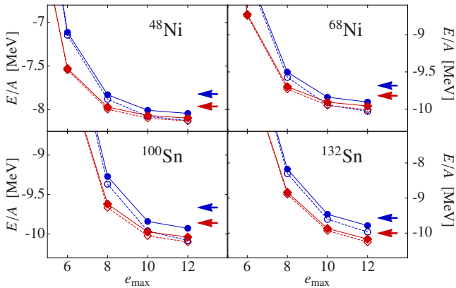
FIG. 3: (Color online) Convergence of CR-CC(2,3) (full symbols) and ACCSD(T) (open symbols) ground-state energies for the NN+3N -full Hamiltonian at \alpha = 0.04 \text{ fm}^4 (blue circles) and 0.08 \text{ fm}^4 (red diamonds), and with E_{3\text{max}} = 14 and \hbar\Omega = 24 \text{ MeV} . Also shown are CCSD ground-state energies (arrows) from e_{\text{max}} = 12 model spaces, where the upper (blue) arrows correspond to \alpha = 0.04 \text{ fm}^4 .
