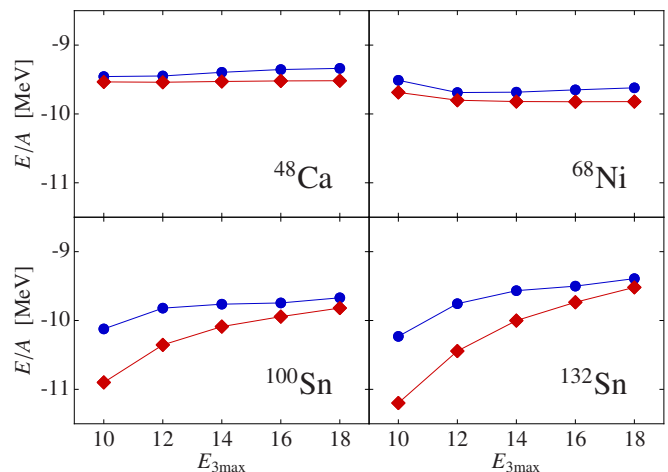
FIG. 4: (Color online) Convergence of CCSD ground-state energies from e_{\text{max}} = 12 CC model spaces, for the NN+3N -full Hamiltonian at \alpha = 0.04 \text{ fm}^4 (blue circles) and 0.08 \text{ fm}^4 (red diamonds) with respect to E_{3\text{max}} . Other parameters of the Hamiltonian as in Fig. 3.
