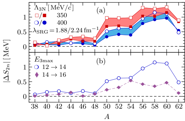
FIG. 3. Uncertainty of Ca two-neutron separation energies: (a) variation as E_{3\max} = 12 \rightarrow 14 for different \Lambda_{3N} and \lambda_{\text{SRG}} = 1.88 to 2.24 \text{fm}^{-1} . (b) Variation E_{3\max} = 12 \rightarrow 14 \rightarrow 16 for \Lambda_{3N} = 400 MeV/c, \lambda_{\text{SRG}} = 1.88 \text{fm}^{-1} .
