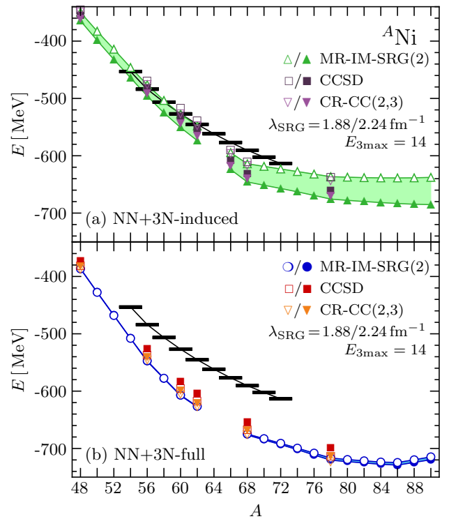
FIG. 4. Ground-state energies of the Ni isotopes for the NN+3N-induced (a) and NN+3N full (b) Hamiltonians, for resolution scales \lambda_{\text{SRG}} = 1.88 to 2.24 \text{fm}^{-1} (open symbols) to 2.24 \text{fm}^{-1} (solid symbols). Experimental data are taken from [50].
