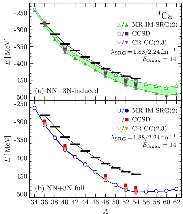
FIG. 1. Ground-state energies of the Ca isotopes for the NN+3N-induced (a) and NN+3N full (b) Hamiltonians, with \lambda_{\text{SRG}} = 1.88 \text{ fm}^{-1} (open symbols) to 2.24 \text{ fm}^{-1} (solid symbols). The band for the MR-IM-SRG(2) results indicate the variation of the results with the resolution scale \lambda_{\text{SRG}} . Experimental data are taken from [26, 50].
