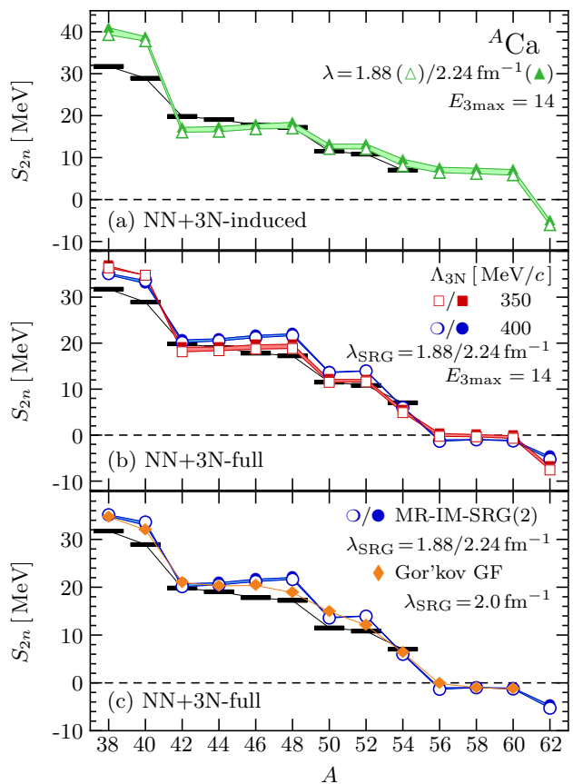
FIG. 2. Two-neutron separation energies of the Ni isotopes for the NN+3N-induced (a) and NN+3N-full Hamiltonian with \Lambda_{3\text{N}} = 350, 400 MeV/c (b), for a range \lambda_{\text{SRG}} = 1.88 to 2.24 fm ^{-1} (open symbols) to 2.24 fm ^{-1} (solid symbols). Panel (c) compares MR-IM-SRG(2) and second-order GGF [6–8] results with the same input Hamiltonian, but slightly different SRG evolution [54]. Experimental values are taken from [26, 50].
