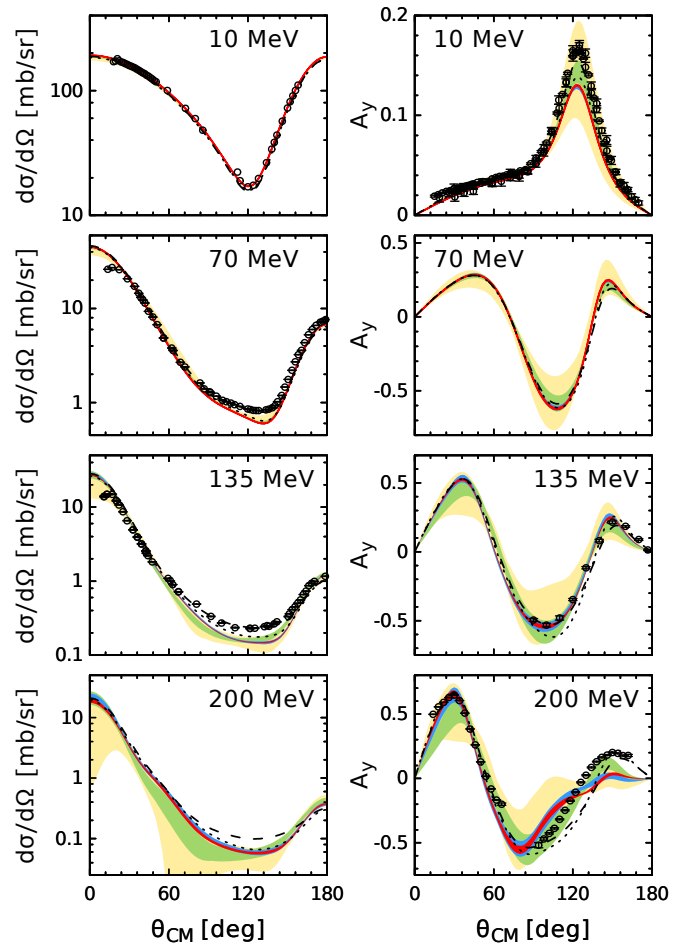
FIG. 3: (Color online) Predictions for the differential cross section and nucleon A_y in elastic Nd scattering based on the NN potentials of Refs. [15, 16] for R = 1.0 fm without including the 3NF. Theoretical uncertainties are estimated via Eqs. (4) and (5) for chiral order i = 2 and via Eqs. (6) and (7) for i \geq 3 . The bands of increasing width show estimated theoretical uncertainty at N^4 LO (red), N^3 LO (blue), N^2 LO (green) and NLO (yellow). The dotted (dashed) lines show the results based on the CD Bonn NN potential [18] (CD Bonn NN potential in combination with the Tucson-Melbourne 3NF [19]). For references to proton-nucleon data (symbols) see Ref. [5].
