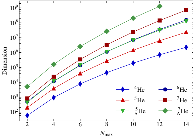
FIG. 3. (Color online) Dimension of the full NCSM model space for natural parity and M_J = \{0, 1/2\} as function of N_{\max} for the two hypernuclei {}^5_{\Lambda}\text{He} and {}^7_{\Lambda}\text{He} , compared to their nucleonic parents and the nuclei obtained by replacing the hyperon with a neutron.
