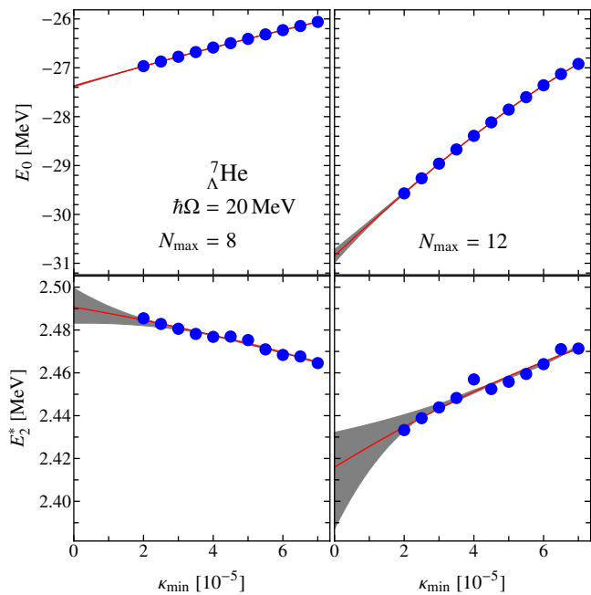
FIG. 4. (Color online) Threshold extrapolation of the absolute ground-state energy and the excitation energy of the second excited state in {}^7_{\Lambda}\text{He} . The computed values (blue dots) are shown together with the best-fit polynomial (red line) and the uncertainty due to the unknown functional form, approximated by a set of different fit polynomials (gray band, see text for details). The regulator cutoff of the YN interaction is \Lambda = 700 \text{ MeV}/c .
