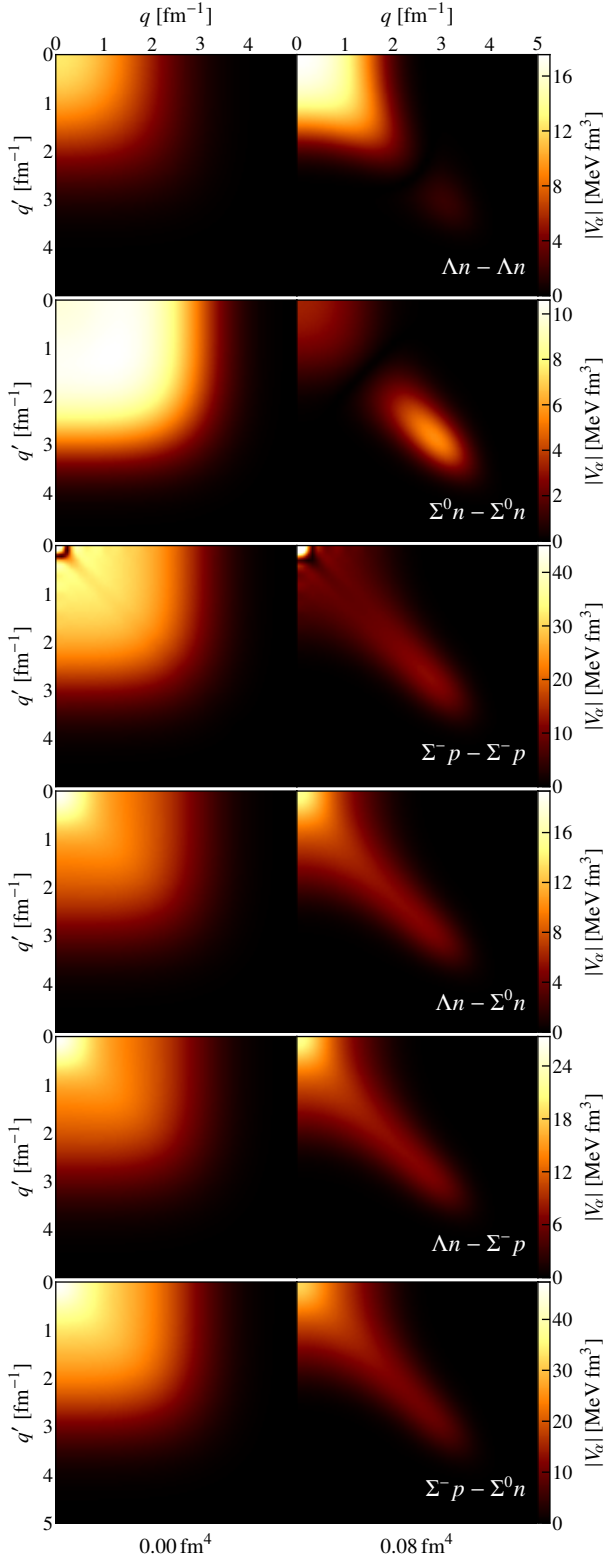
FIG. 1. (Color online) Momentum-space matrix elements of the Q = 0 , S = -1 ^1S_0 partial wave for the bare and evolved hypernucleon interaction. The particle-combinations are coupled by the transition matrix elements in the right column and have to be evolved simultaneously. The low-momentum matrix elements of the \Sigma^- p channel (third row) are dominated by the Coulomb interaction.
