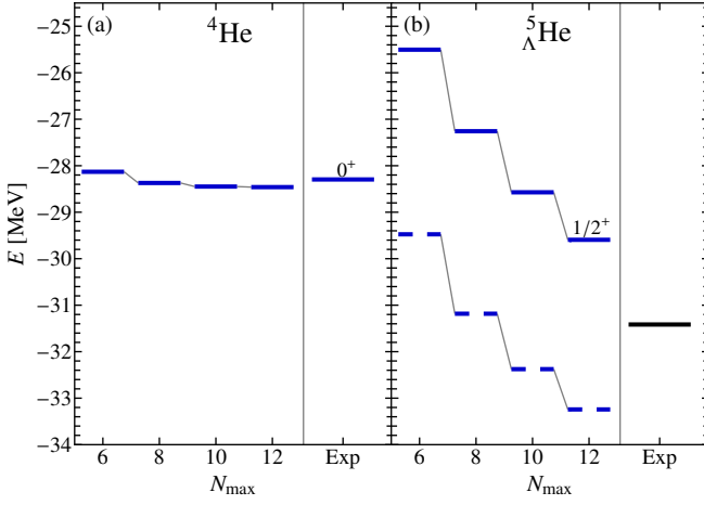
FIG. 6. (Color online) Absolute ground-state energy of (a) {}^4\text{He} and (b) its daughter hypernucleus {}^5_{\Lambda}\text{He} . The oscillator frequency is \hbar\Omega = 20 MeV, the flow parameters in the nucleonic and hyperonic sectors are \alpha_N = 0.08 \text{ fm}^4 and \alpha_Y = 0 \text{ fm}^4 , respectively. The regulator cut-offs employed are \Lambda = 700 \text{ MeV}/c (solid lines) and \Lambda = 600 \text{ MeV}/c (dashed lines). Experimental data from Refs. [3, 63].
