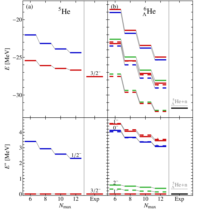
FIG. 7. (Color online) Absolute and excitation energies of low-lying states in (a) {}^5\text{He} and (b) its daughter hypernucleus {}^6_{\Lambda}\text{He} . Parameters are the same as in Fig. 6. Vertical lines mark extrapolation uncertainties, experimental data taken from Refs. [3, 63].
