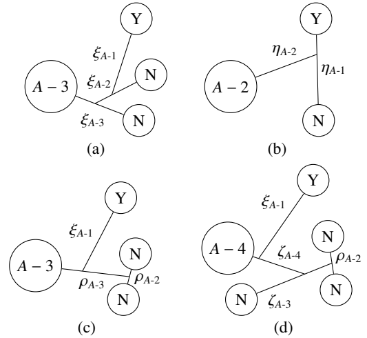
FIG. 2. Illustration of the Jacobi coordinates used for (a) antisymmetrization and embedding of the (b) YN , (c) NN , and (d) NVN interactions.
