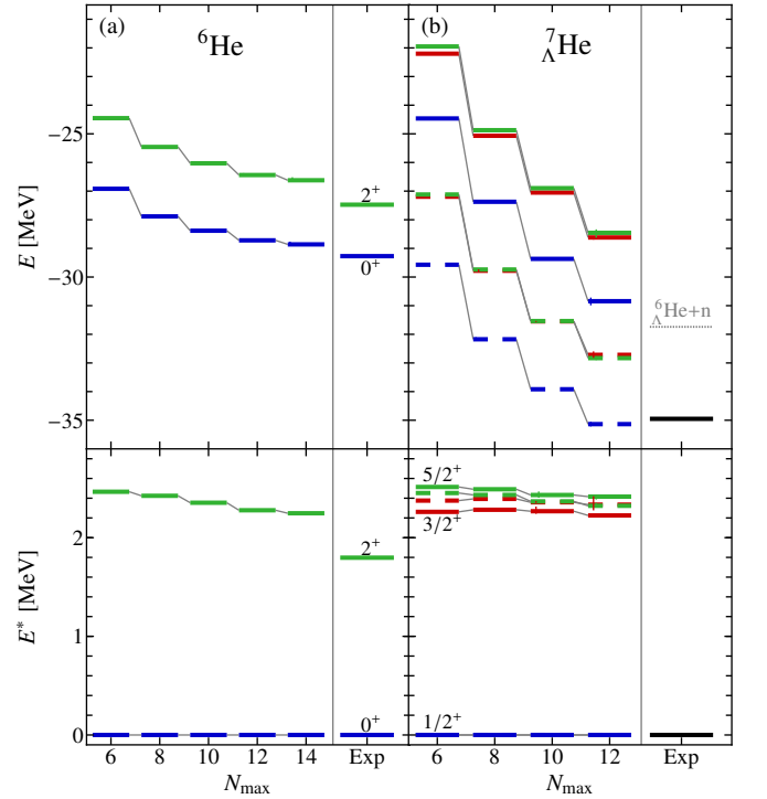
FIG. 8. (Color online) Absolute and excitation energies of low-lying states in (a) {}^6\text{He} and (b) its daughter hypernucleus {}^7_{\Lambda}\text{He} . Parameters are the same as in Fig. 6. Vertical lines mark extrapolation uncertainties, experimental data taken from Refs. [7, 63].
