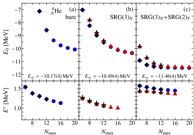
FIG. 5. (Color online) Ground-state and excitation energy of {}^4_\Lambda\text{He} for the (a) bare, (b) \text{SRG}(3)_N evolved to \alpha = 0.04 \text{ fm}^4 (red triangles) and \alpha = 0.08 \text{ fm}^4 (blue circles), and (c) \text{SRG}(3)_N + \text{SRG}(2)_Y Hamiltonian, obtained from a J-NCSM calculation. The regulator cutoff is \Lambda = 600 \text{ MeV}/c , the basis frequency is \hbar\Omega = 20 \text{ MeV} for the evolved Hamiltonians and \hbar\Omega = 30 \text{ MeV} for the bare one. The crosses denote the IT-NCSM results for both flow parameters, E_\infty is the energy extrapolated to N_{\text{max}} \rightarrow \infty .
