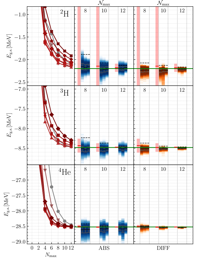
Figure 4: Input data and predicted ground-state energies for {}^2\text{H} , {}^3\text{H} and {}^4\text{He} . The left-hand column shows the input data for multiple HO frequencies around the variational minimum. In the middle and right-hand columns show the statistical predictions are shown as color-coded vertical histograms at a given \mathcal{N}_{\max} . The groups of three histograms corresponds to the filters (a) to (c) on the training data (see text for details). The networks were trained and evaluated with either the ABS (middle) or DIFF (right) mode. The dashed black lines (---) are the variational boundaries for the respective model space and the horizontal green line (—) indicates the converged value. For comparison classical extrapolations are given as red bars with uncertainty bands (—).
