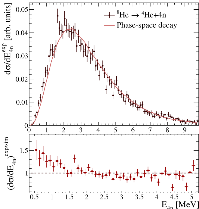
FIG. 5. Top: 4n relative-energy spectrum ( E_{4n} ) for {}^8\text{He} \rightarrow {}^4\text{He} + 4n breakup channel. The red curve represents a simulated distribution assuming 5-body phase-space decay. Bottom: measured E_{4n} distribution divided by the simulated one.
