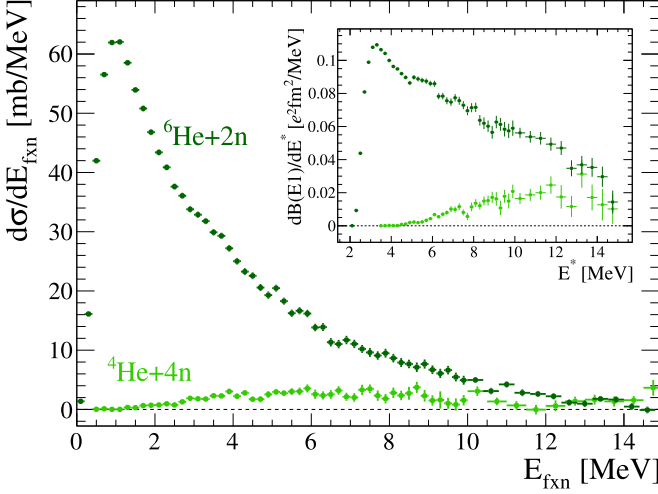
FIG. 2. Coulomb excitation cross section spectra for three- (dark green) and five-body (light green) breakup channels of ^8\text{He} measured with lead target. The inset shows the corresponding dipole strength distributions, dB(E1)/dE^* , as a function of the excitation energy.
