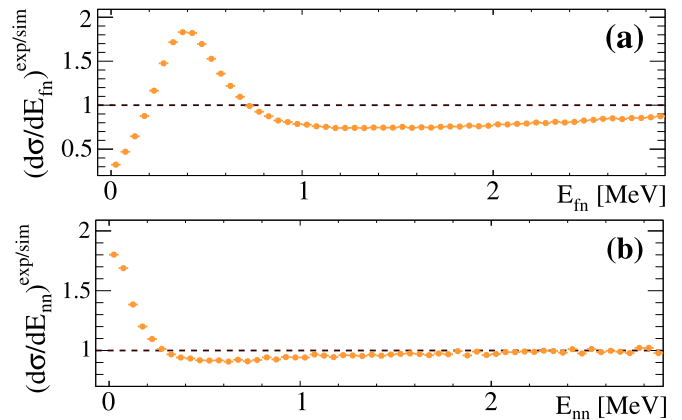
FIG. 4. (a) Fragment-neutron ( fn ) two-body relative energy ( E_{fn} ) for ^8\text{He} \rightarrow ^6\text{He} + 2n breakup channel. Shown is the measured spectrum divided by a simulated one assuming phase-space decay. (b) Same for the neutron-neutron sub-system.
