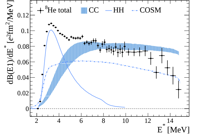
FIG. 3. Total B(E1) spectrum measured with lead target. Theory predictions folded with the experimental response are shown in blue based on CC [14] (band), HH [37] (solid curve) and COSM [38] (dotted-dashed curve).
